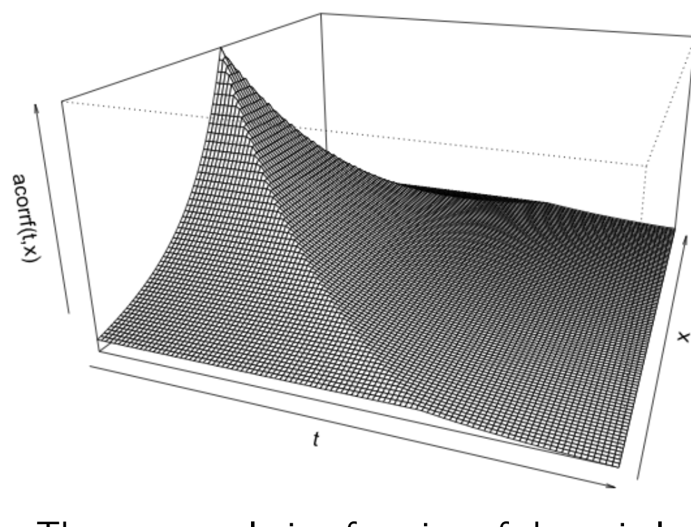
The autocorrelation function of the strictly stationary solution in the example: \text{acorf}(t, x) = \min(\exp(-\lambda t), \exp(-\frac{\lambda \|x\|}{c}))
